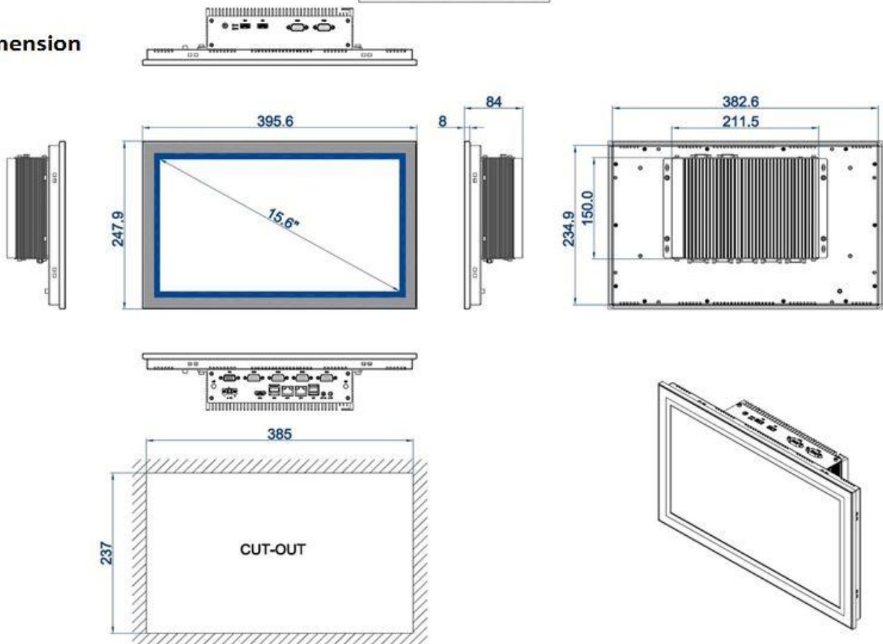
DIMENSIONAL DRAWING:TPC-PR156
